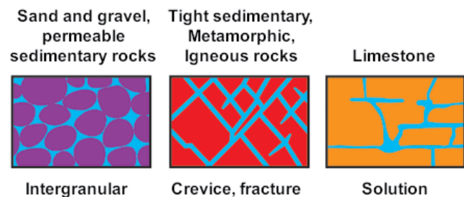
Figure 4. Main types of porosity and permeability.
