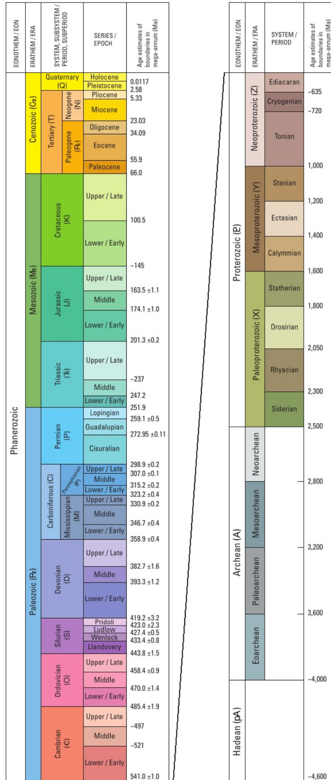
Figure 10: Geologic time scale.
