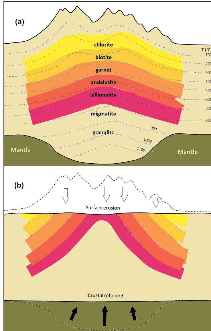
Figure 19: Schematic cross-section through the Meguma Terrane, showing: (a) metamorphic zones and temperatures when mountain-building processes thickened the crust, and (b) after the mountains have been eroded, exposing at surface metamorphic rocks that formed deep within the mountains. The colours representing metamorphic zones are per Figure 17. (modified from Panchuk, 2024)
