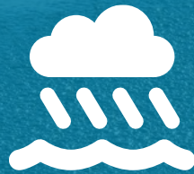
Extreme Storms
