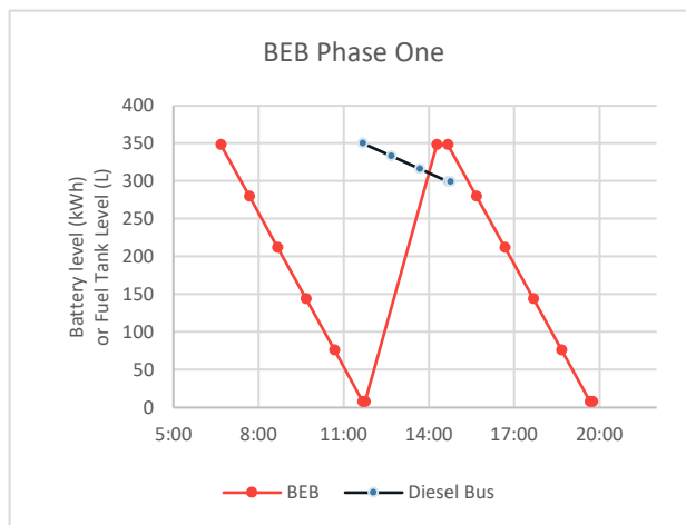
Figure C: Battery Level for BEB
